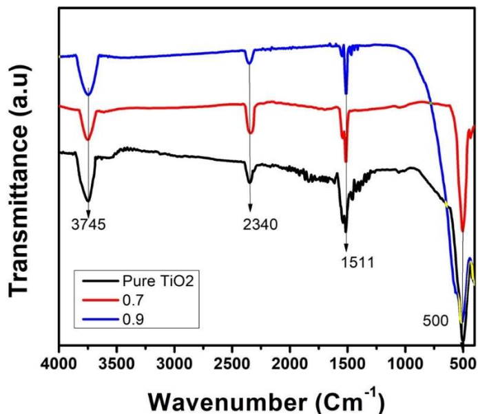
Fig. 2: The FTIR spectra of pure TiO 2 , 0.7%, and 0.9% MFTNc all display distinctive vibrational peaks. O-H stretching vibrations, which indicate surface-adsorbed water or hydroxyl groups, are represented by the broadband at about 3745 cm -1 . The band at 1511 cm -1 is linked to C=C aromatic stretching, which may be caused by phytochemical residues, whereas the peak at 2340 cm -1 is ascribed to CO 2 adsorption. The anatase phase of TiO 2 is confirmed by the strong band near 500 cm -1 , which represents Ti–O–Ti lattice vibrations. These bands are slightly shifted and sharpened by doping, indicating successful surface modification and Fe incorporation.
